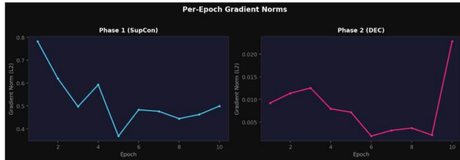
Figure 4.7: Per-epoch gradient norms for exp02.
