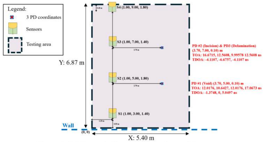
Figure 3.7: Schematic diagram of experimental layout.
