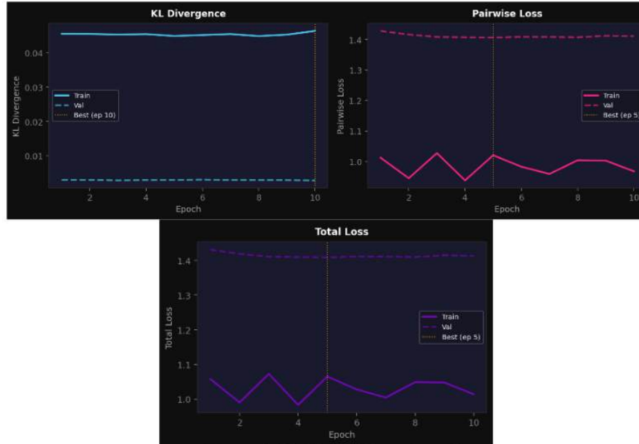
Figure 4.20: Phase 2 loss of exp03.
