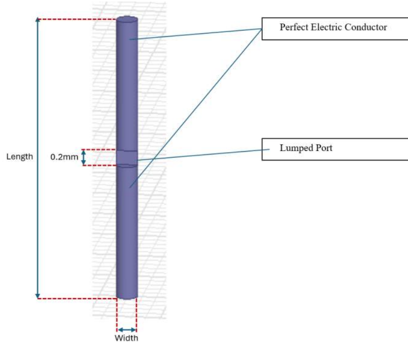
Figure 3.3: Shape and materials assigned to the PD model (dipole antenna).
