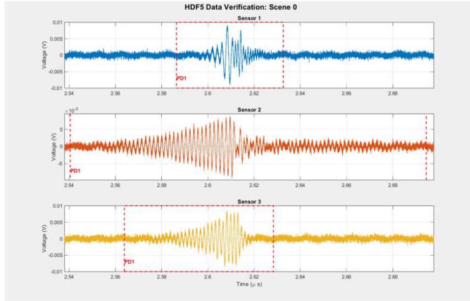
Figure 3.5: Simulated waveforms using HFSS and MATLAB.
