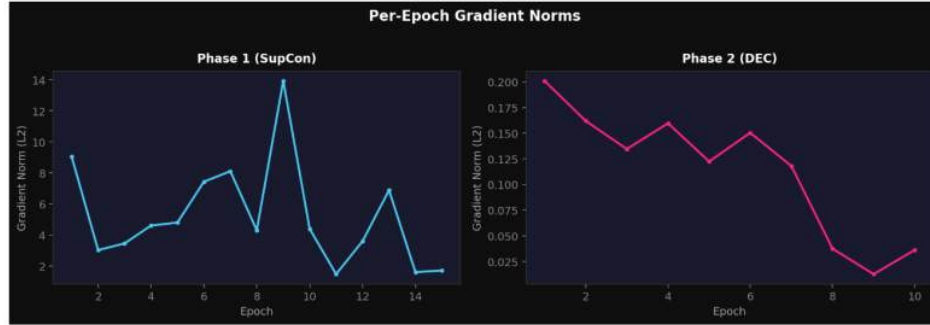
Figure 4.18: Per-epoch gradient norms of exp03.
