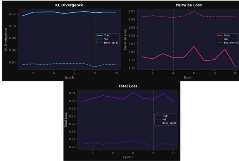
Figure 4.9: Phase 2 Loss for exp02.
