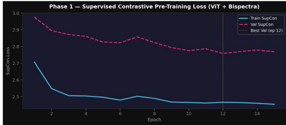
Figure 4.19: Phase 1 loss for exp03.
