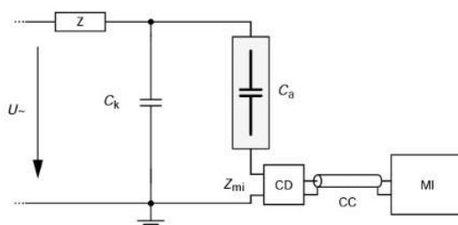
Figure 1.1: Traditional method of measuring PD occurrence (IEC60270:2025).
