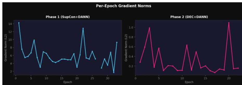
Figure 4.30: Per-epoch gradient norms for exp04.
