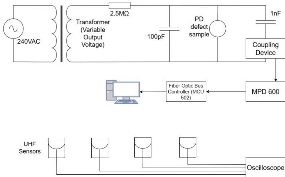
Figure 3.9: Circuit Diagram of Experiment.
