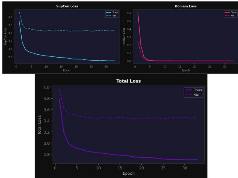
Figure 4.31: Phase 1 loss for exp04.
