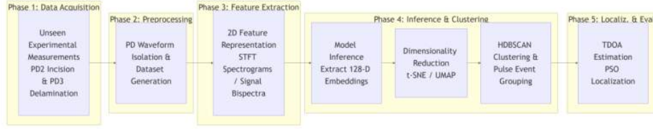
Figure 3.2: Model testing and localization pipeline.
