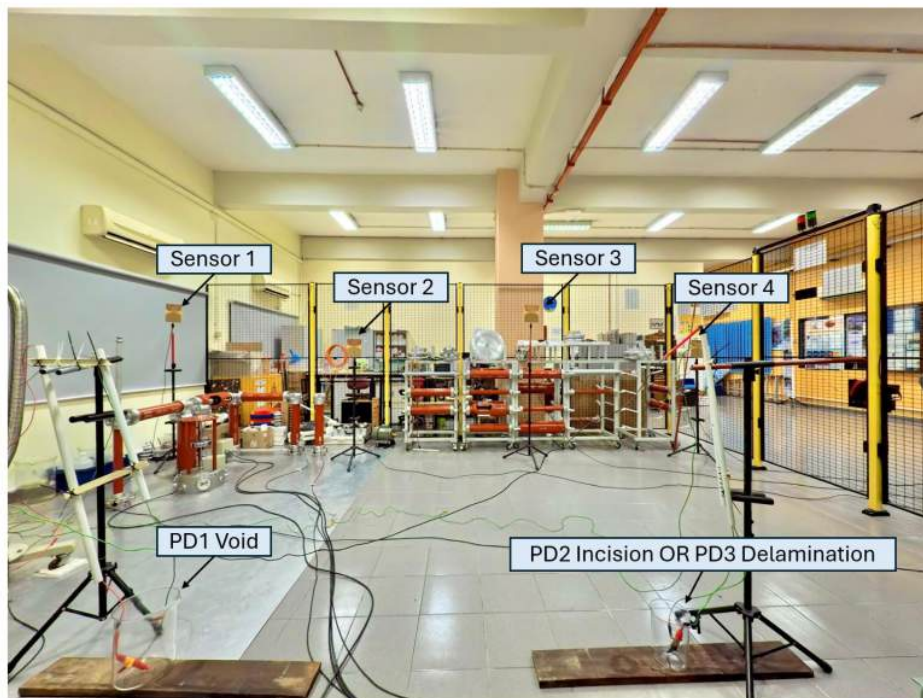
Figure 3.8: Actual experimental layout.
